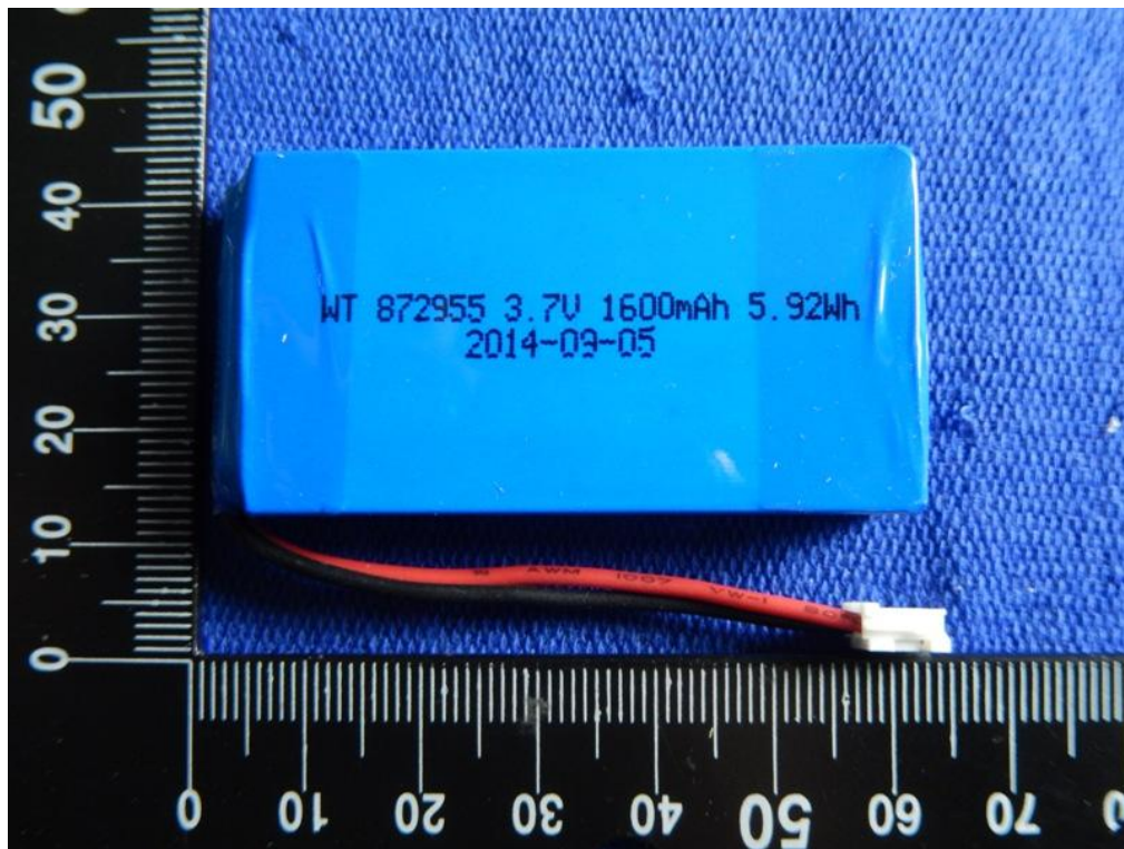
Battery (WT872955 3,7V 1600mAh 5,92Wh)
